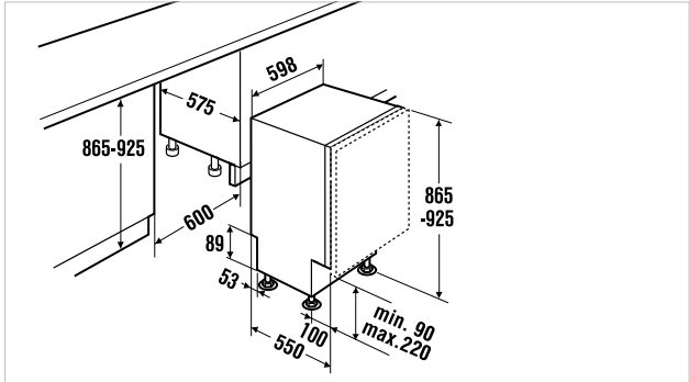
IGVS 6506.3 fully-integrated
